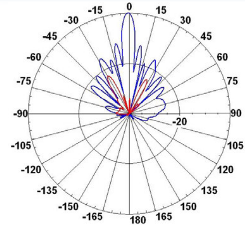
5.5 Ghz E-Plane and H of E-Plane
